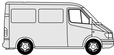
Sprinter 04/00 → 03/06
