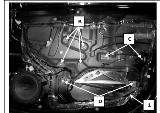
Porta lato destro, Portière avant droite, Right front door, Puerta lado derecho, Vorne rechte Tür, Porta frente dijeta, Sag on kapi, πόρτα εμπρόςθια δεξιά
