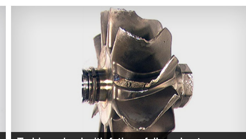
Turbine wheel with fatigue failure due to cyclic overspeed
