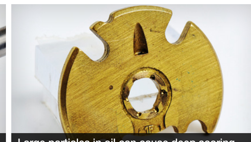
Large particles in oil can cause deep scoring and impacts
