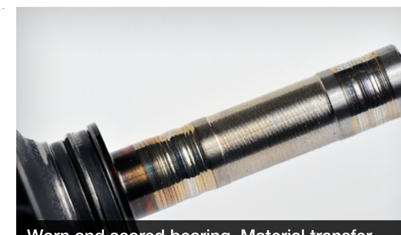
Worn and scored bearing. Material transfer to the shaft
