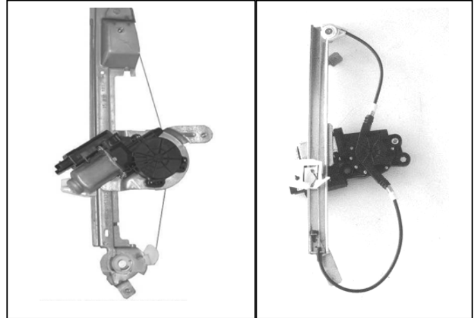
Elevalunas original Oem window regulator
