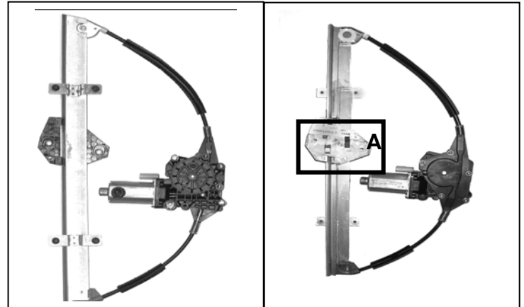
Elevavinas original Oem window regulator
