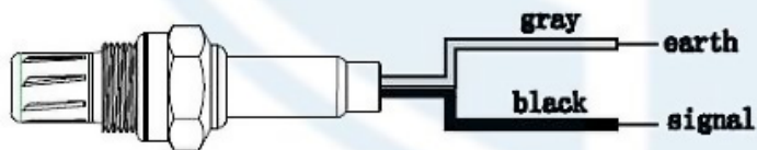
two wires
