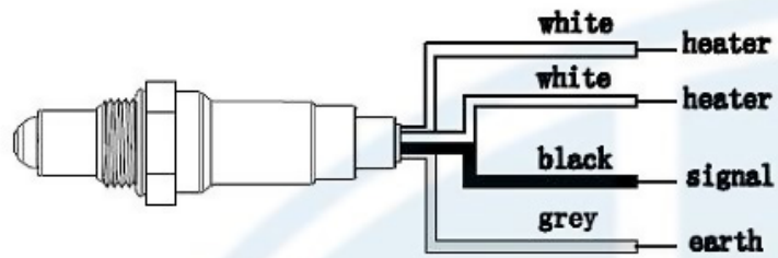
four wires
