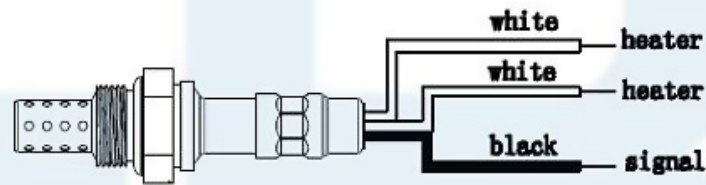
three wires
