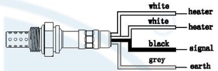
four wires
