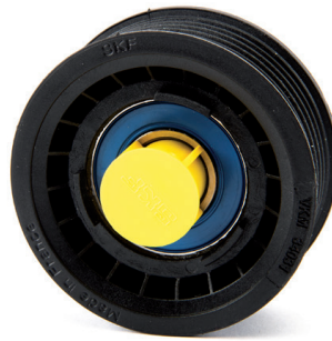
Fig. 1: 532 0471 10 - old design
