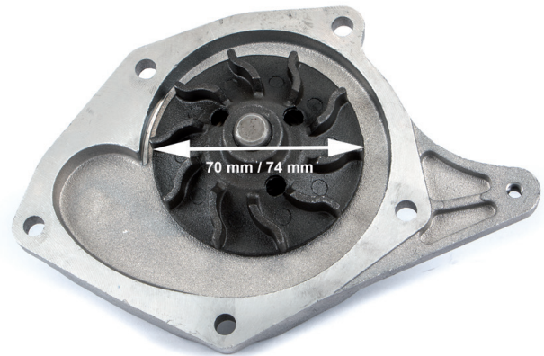
Determining the impeller diameter after removal of the coolant pump
