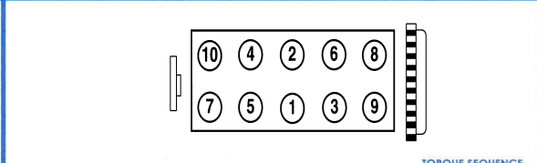
TORQUE SEQUENCE
