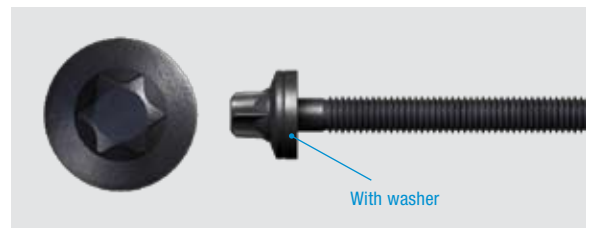
Fig. 1_Old/replaced bolt with washer (OE No. 607 926)
