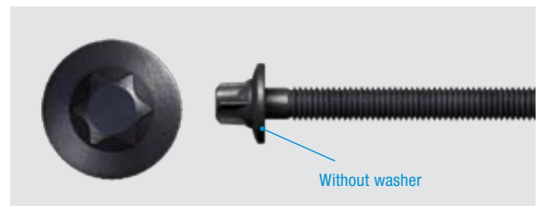
Fig. 2_New bolt without washer (OE No. 65 07 937)
